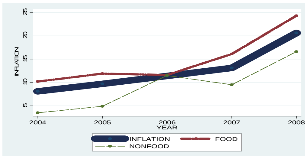
Figure 2.1: Inflationary dynamics: 2004-2008
